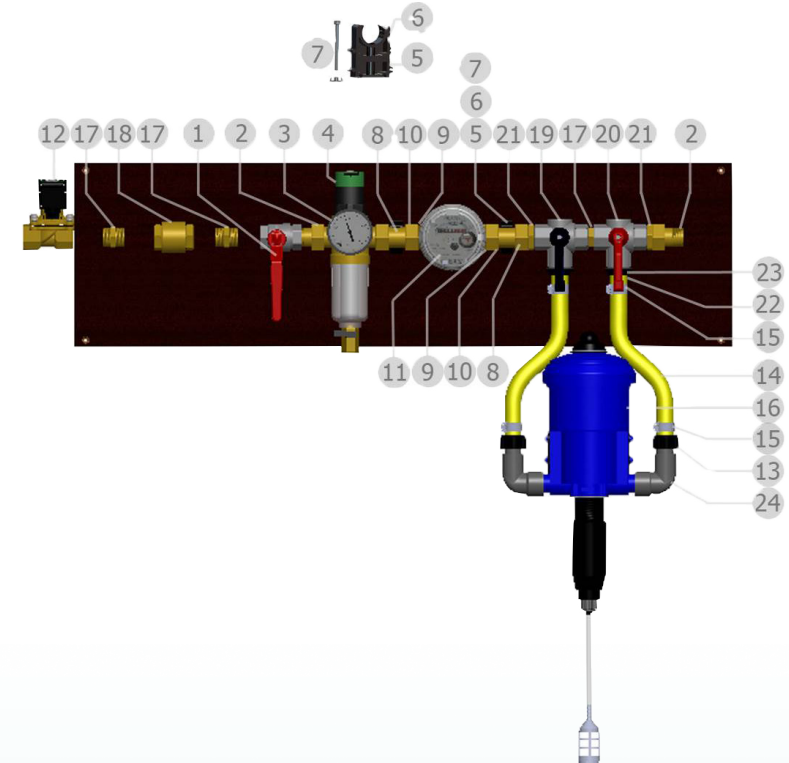
Position ball valve With Dosatron
